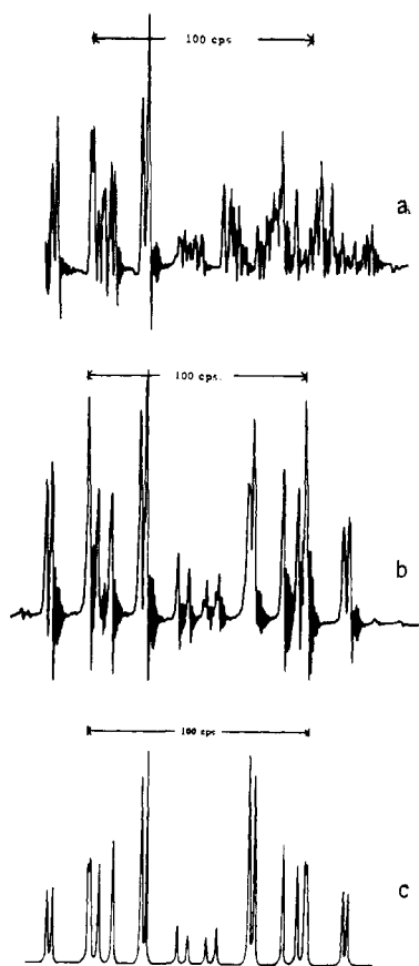
Figure 1. Fluorine nuclear magnetic resonance spectrum at 56.4 Mc.p.s. of (a) 1,1,4,4-tetrafluoro-1,3-butadiene, (b) ^{19}\text{F}\{-^1\text{H}\} spectrum, and (c) calculated ^{19}\text{F}\{-^1\text{H}\} spectrum.
