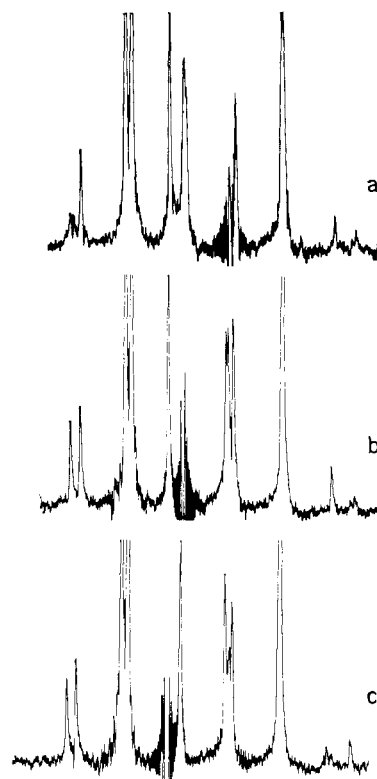
Figure 4. High-field portion of the 56.4-Mc.p.s. ^{19}\text{F}\{-^1\text{H}_m\} nuclear magnetic resonance spectrum of bis-4,5-(difluoromethylene)cyclohexene with fluorine-fluorine decoupling: (a) line 6 irradiated, (b) line 7 irradiated, (c) line 8 irradiated.
