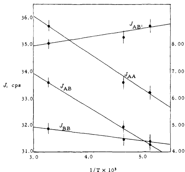
Figure 6. Temperature dependence of F-F coupling constants in 1,1,4,4-tetrafluoro-1,3-butadiene, J_{AA} and J_{AB} left scale, J_{AB'} and J_{BB} right scale.
