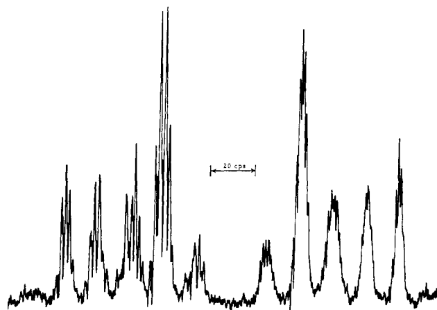
Figure 2. Fluorine nuclear magnetic resonance spectrum at 56.4 Mc.p.s. of bis-4,5-(difluoromethylene)cyclohexene.
