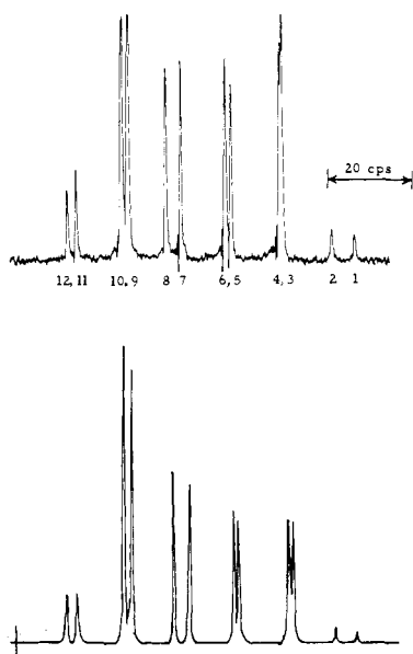
Figure 3. High-field half of the 56.4-Mc.p.s. ^{19}\text{F}\{-^1\text{H}\} nuclear magnetic resonance spectrum of bis-4,5-(difluoromethylene)cyclohexene: (a) observed, (b) calculated.
